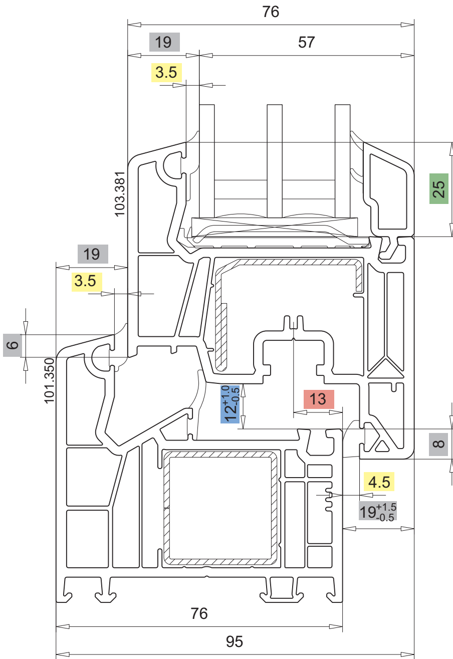
Systemmaße SOFTLINE 76 [mm]
